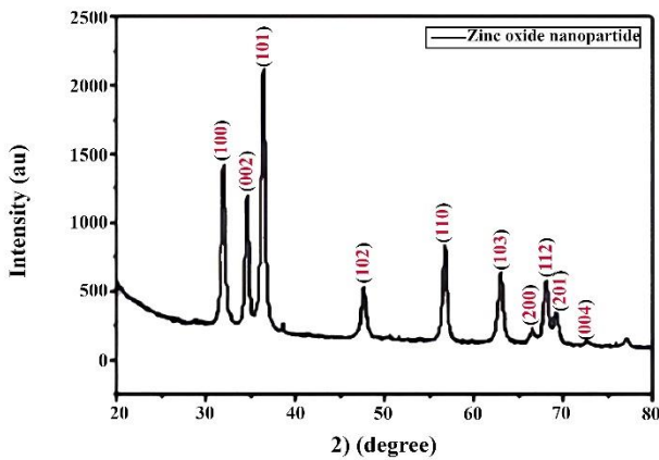
Fig. 4 X-ray refraction analysis of zinc oxide nanoparticles.
